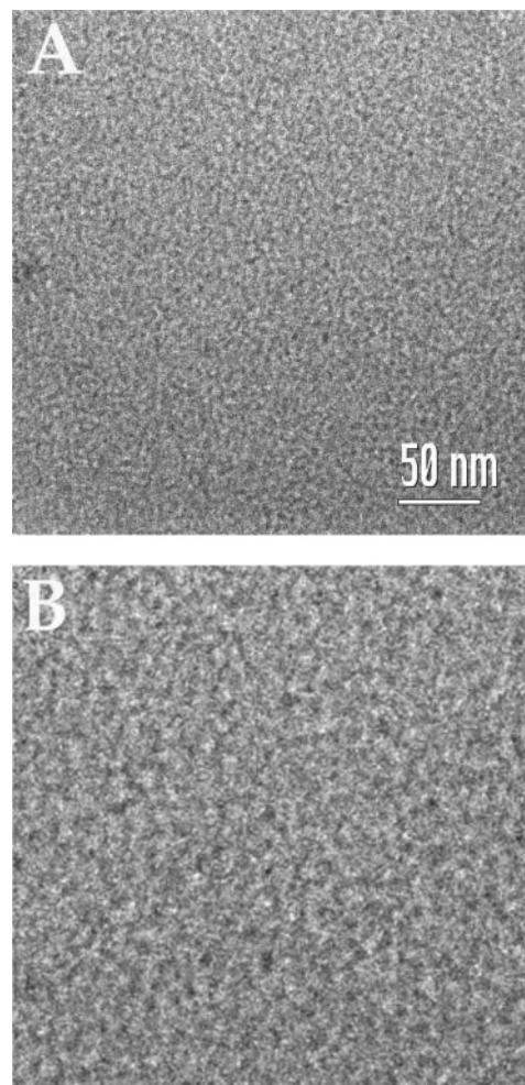
Figure 1. (A) Cryo-TEM image of spheroidal micelles found in the reaction mixture of SBA-15, taken after a reaction time of 8.5 min, vitrified from 50 °C. (B) Same area at double the magnification of A.
